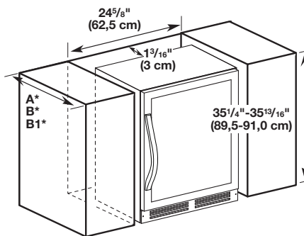
WUW35X24DS WUW55X24DS
